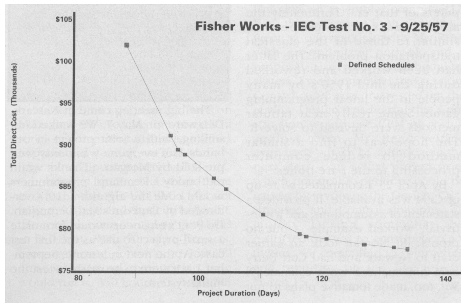
Fig. 10 Cost v Duration derived from CPM modelling. (Kelley and Walker, 1989, p9)
